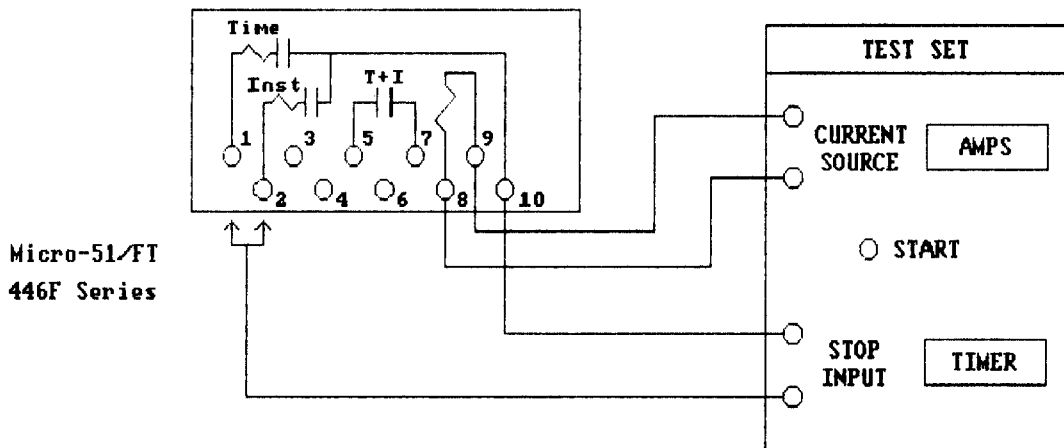
Figure 6b: Typical Test Connections - Micro-51/FT
