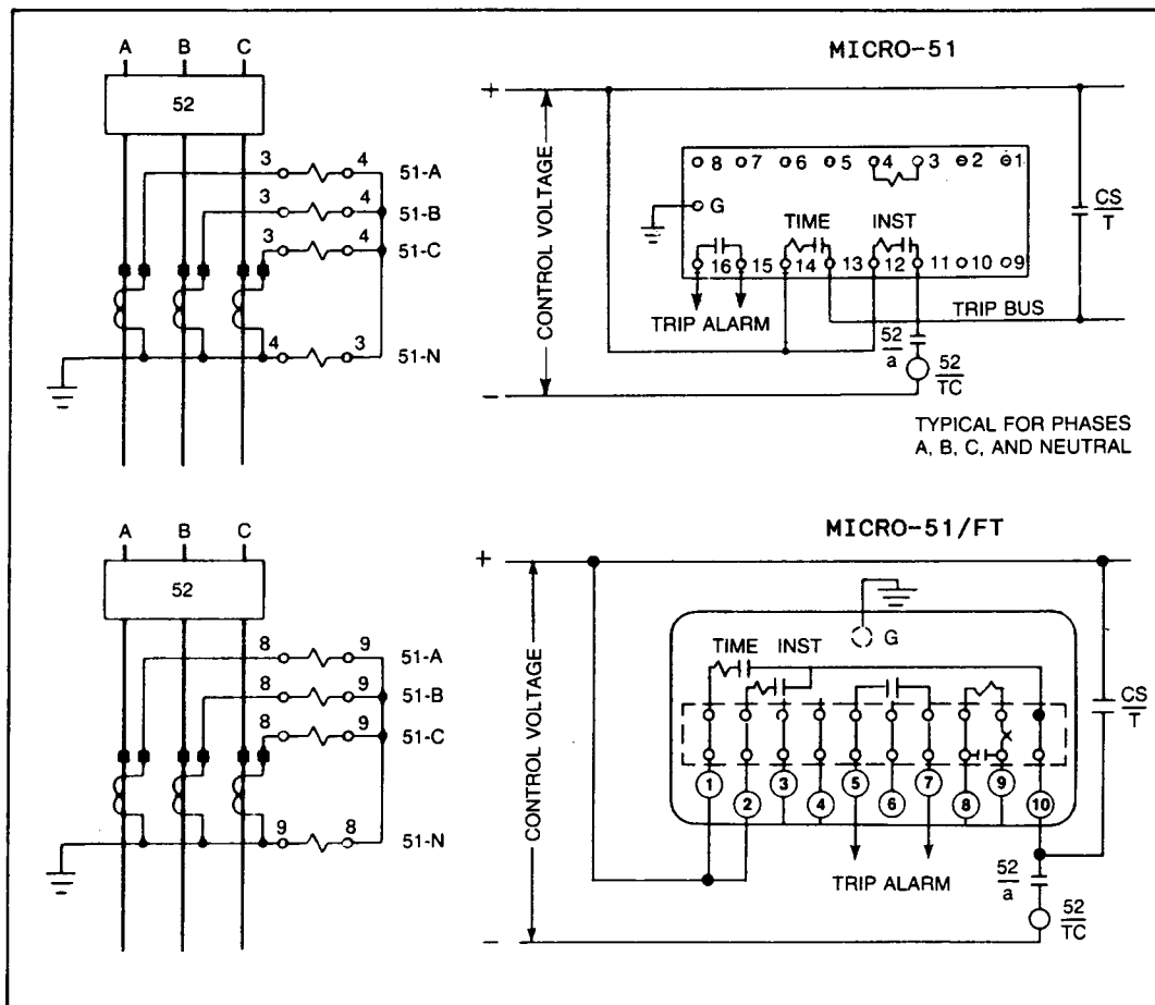
Figure 3a: Typical External Connections Three-phase and Ground Overcurrent Protection
