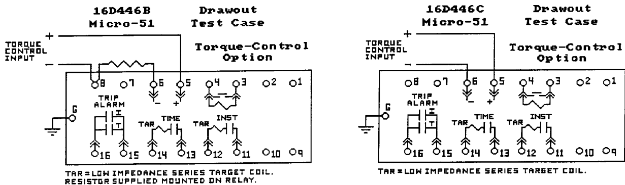
Figure 2b: Internal Connections - Torque-Control Models
