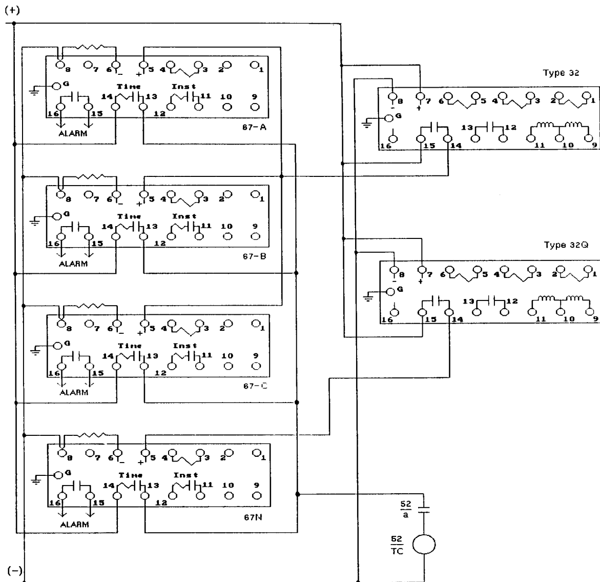
Figure 3b: Typical Control Connections - Micro-51 used with Circuit-Shield Types 32 and 32Q in a Directional Phase and Ground Overcurrent Scheme
