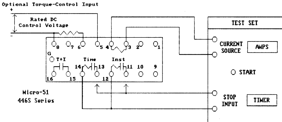
Figure 6a: Typical Test Connections - Type Micro-51
