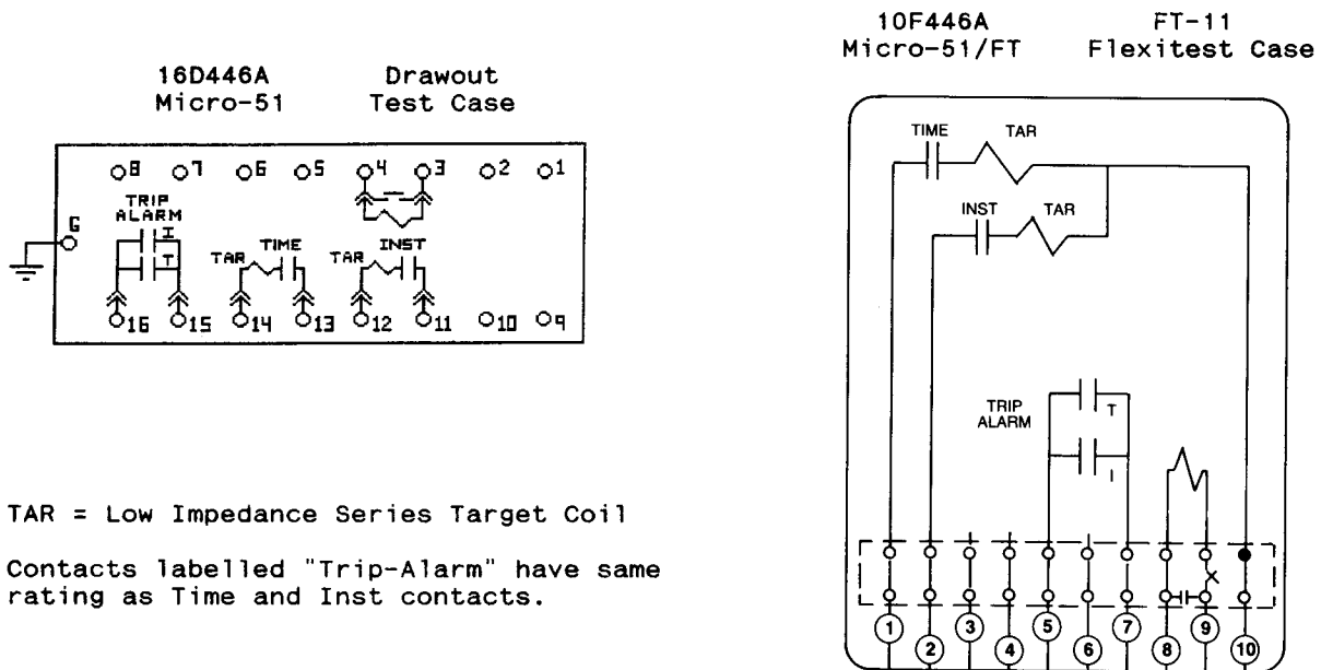
Figure 2a: Internal Connections - Standard Units
