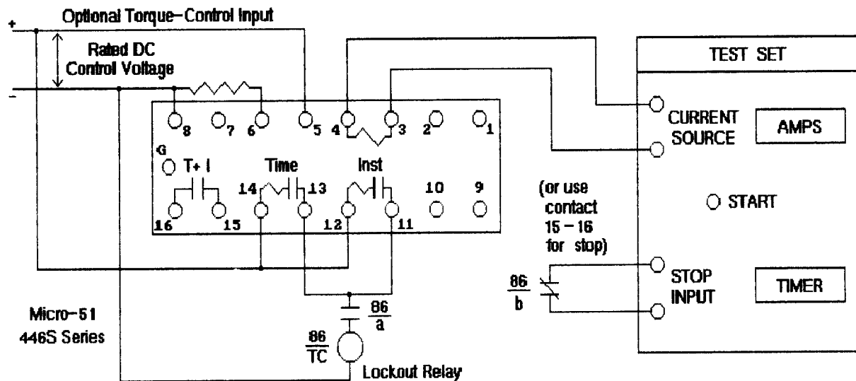
Figure 7: Typical Test Connections - Micro-51 Target Operation Functional Check
