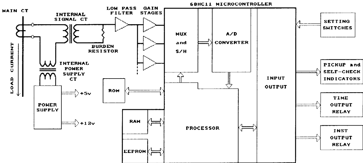
Figure 4: Block Diagram of Micro-51 Time-Overcurrent Relay
